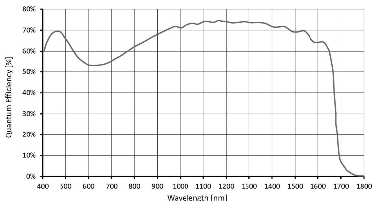
Absolute quantum efficiency of IM992
